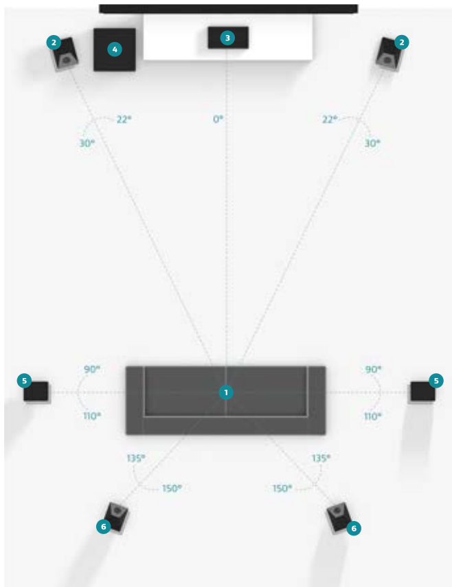
7.1.4 Speaker Placement
