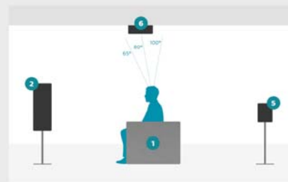
5.1.2 Ceiling Speaker Placement Detail
