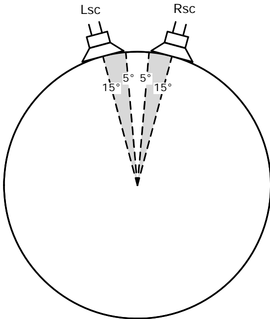
Figure 19: Left Screen and Right Screen speaker placement.
