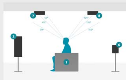
7.1.4 Ceiling Speaker Placement Detail
