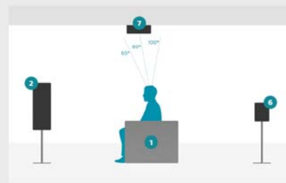
7.1.2 Ceiling Speaker Placement Detail
