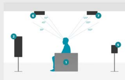
5.1.4 Ceiling Speaker Placement Detail
