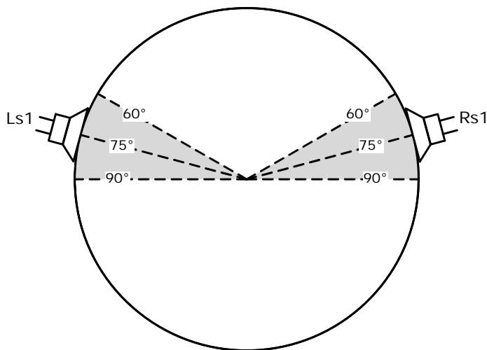
Figure 20: Left Surround 1 and Right Surround 1 speaker placement.
